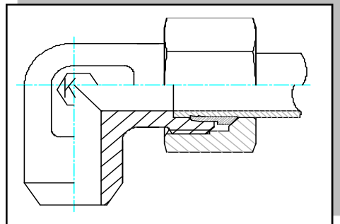
WAS Weld Elbow KAD Kaynaklı Dirsek
