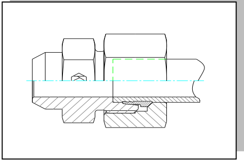
AS Weld Connector KRE Kaynaklı Rekor
