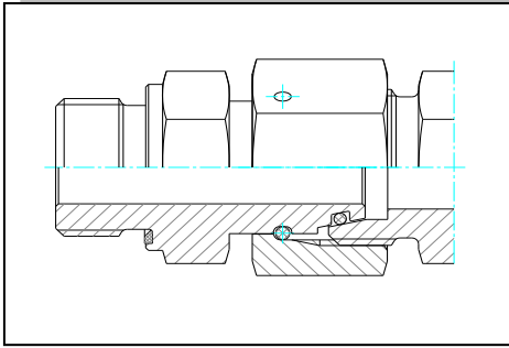
EGE R-M-ED Swivel Connector TRE/P-R-M-PLX Pimli Ters Rekor
