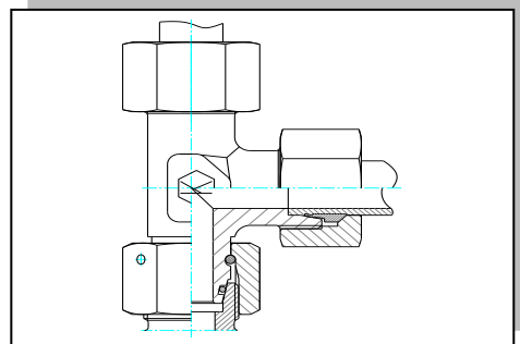
EL Swivel Nut Run Tee YT/P Pimli Yan Bacak Ters T
