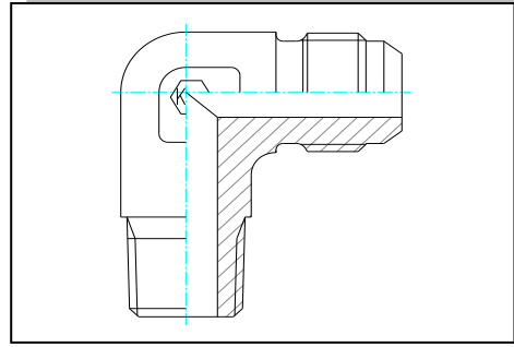
Male Stud Elbow (BSPT) JIC 37° HAD Hortum Ara Dirseği (BSPT) JIC 37°
