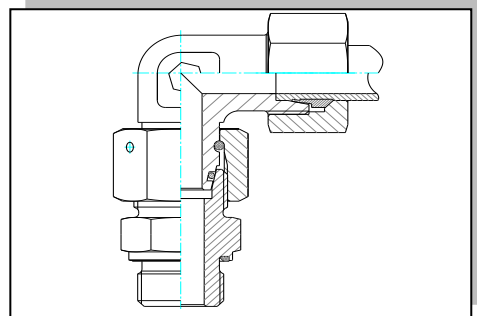
EVW-R-ED Assembled Adjustable Swivel Nut Elbow RTD/P-R Pimli Rekorlu Dirsek
