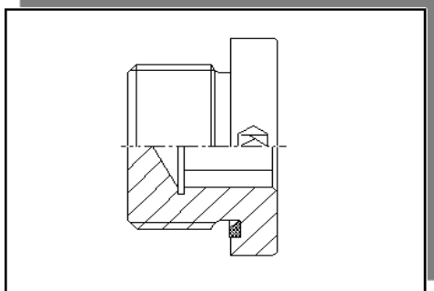
VSTI M/R-ED Blanking plug for ports ALKT-R/M-PLX Peflex'li Alıyanbaşı Körtapa
