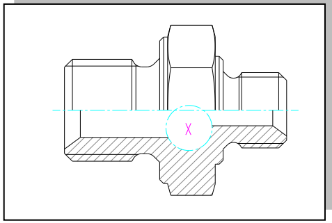
Male to Male Adapters ODZN 30° İç Konik Orantılı Düz Nipel
