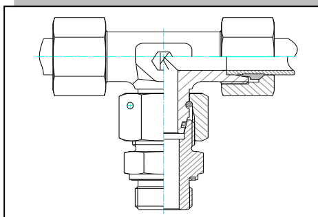
EVT-R-ED Assembled Adjustable Swivel Branch Tee ORT/P-R Pimli Rekorlu Orta Bacak T
