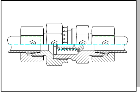
RHD Non Return Valve CVFN Cek Valf Nipeli
