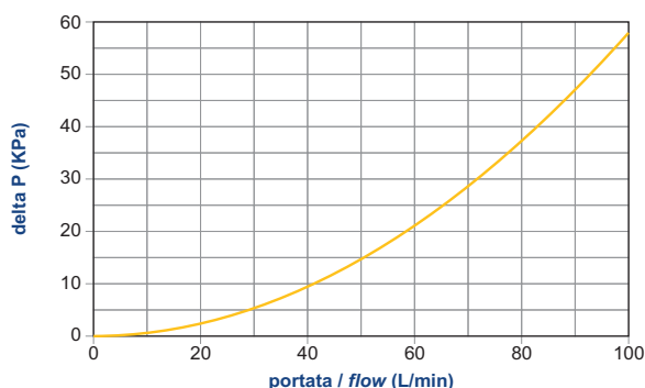
\Delta P CORPI / \Delta P HOUSINGS
